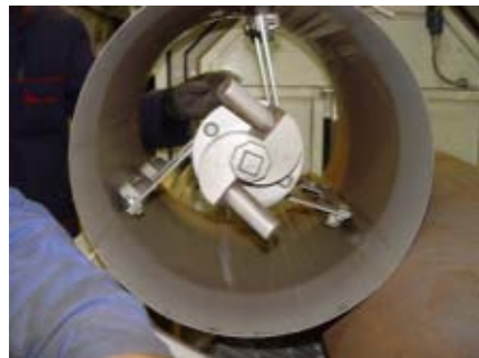
Rotation blasting head
