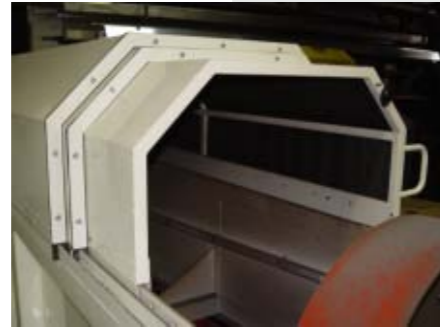
The protective cover enables sandblasting of perforated tubes.
